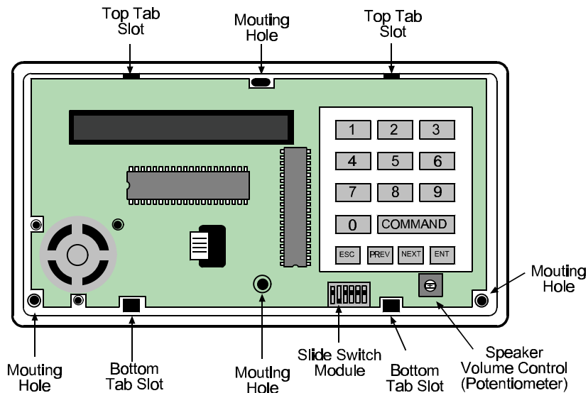
Figure 1: D1255 Internal Features
